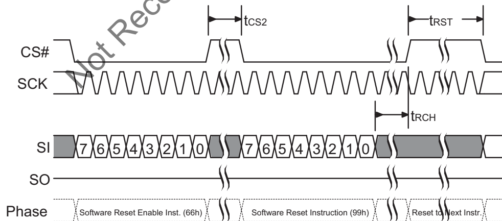
Figure 26. Software Reset Input Timing
